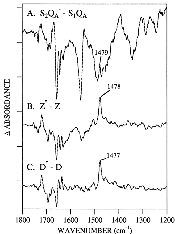
Fig. 5. Difference infrared spectra of Synechocystis PSII preparations. The difference spectra are of (A) S_2Q_A^- - S_1Q_A from oxygen-evolving cyanobacterial PSII, and (B) Z^{\bullet} - Z and (C) D^{\bullet} - D from manganese-depleted cyanobacterial PSII. Data shown in (A) are the average of 2–4 spectra; data shown in (B–C) are the average of 17 spectra. The tick marks on the y axis correspond to 2 \times 10^{-4} absorbance units.
