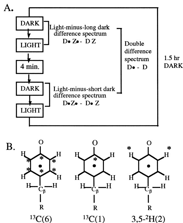
Fig. 3. (A) Schematic of difference FT-IR data collection method for \text{Z} \cdot -\text{Z} and \text{D} \cdot -\text{D} by continuous illumination at -9^{\circ}\text{C} . The boxes labeled 'light' and 'dark' correspond to 4 min of data acquisition. (B) Structures of isotopically labeled tyrosines. Asterisks mark the ^{13}\text{C} or the ^2\text{H} on the tyrosine.
