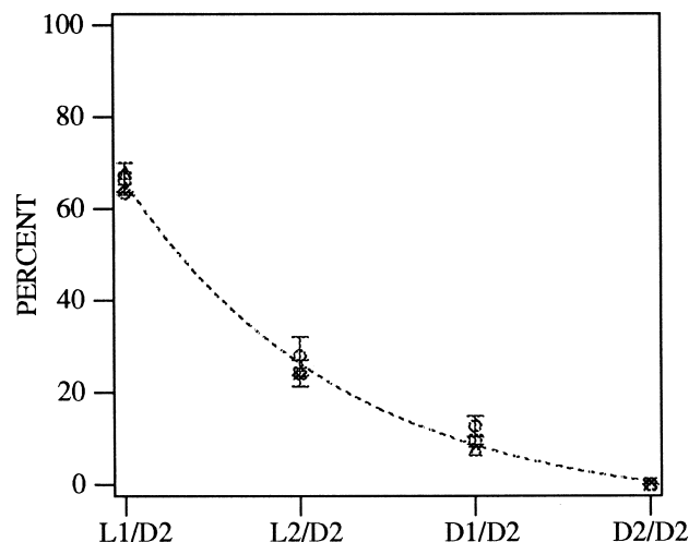
Fig. 11. Decay of tyrosyl D \cdot signals, as assessed by EPR and difference FT-IR spectroscopy, in manganese-depleted spinach PSII preparations. Data plotted are from flash illumination infrared measurements, shown in Fig. 10 (circles). Also plotted are the corresponding, integrated areas from the kinetic EPR decay of tyrosyl D \cdot radical, shown in Fig. 8C (triangles) and Fig. 8D (squares). The best fit to the data points is shown as the dotted line.
