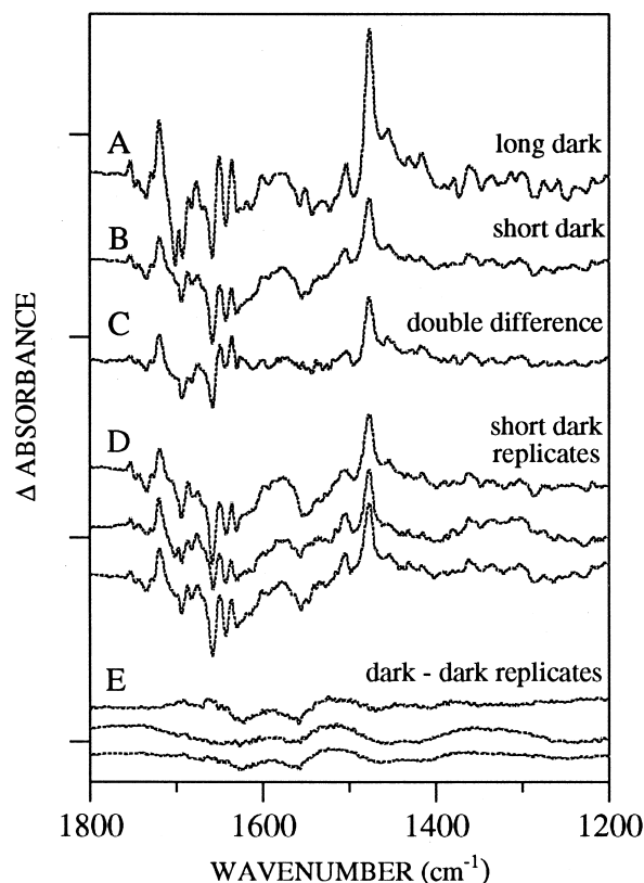
Fig. 4. Difference infrared spectra of manganese-depleted wild-type Synechocystis PSII preparations at pH 7.5. The (A) light-over-long dark, (B) light-over-short dark, and (C) double-difference infrared spectra shown were obtained using continuous illumination, according to the data acquisition methods described in Fig. 3A. Spectra in (A–C) are an average of 17 spectra. Three individual light-minus-dark difference spectra, taken from three different samples on three different days, are shown in (D). The corresponding three individual dark-minus-dark difference spectra are shown in (E). The tick marks on the y axis measure 5 \times 10^{-4} absorbance units. Data were obtained at -9^{\circ}\text{C} .
